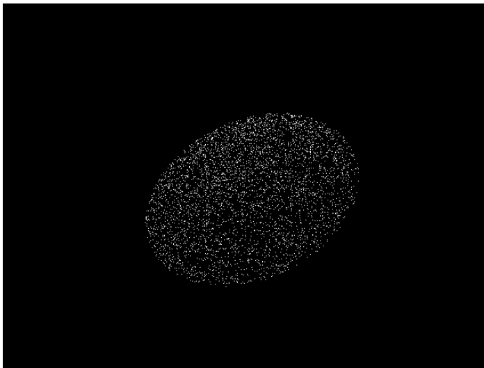
Figure 4.10.4: glm::vec4(glm::diskRand(1.0f), 0, 1);
